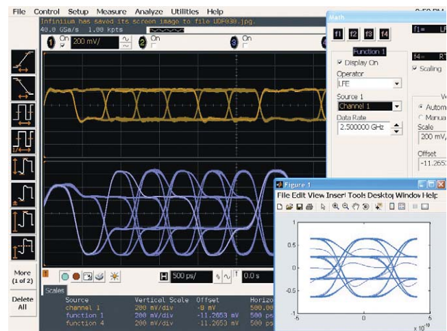
Signal equalization using user-defined function.
