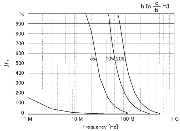
Figure 29. Permeability ( \mu'_r ) vs. frequency (at F = 3 , typical)
